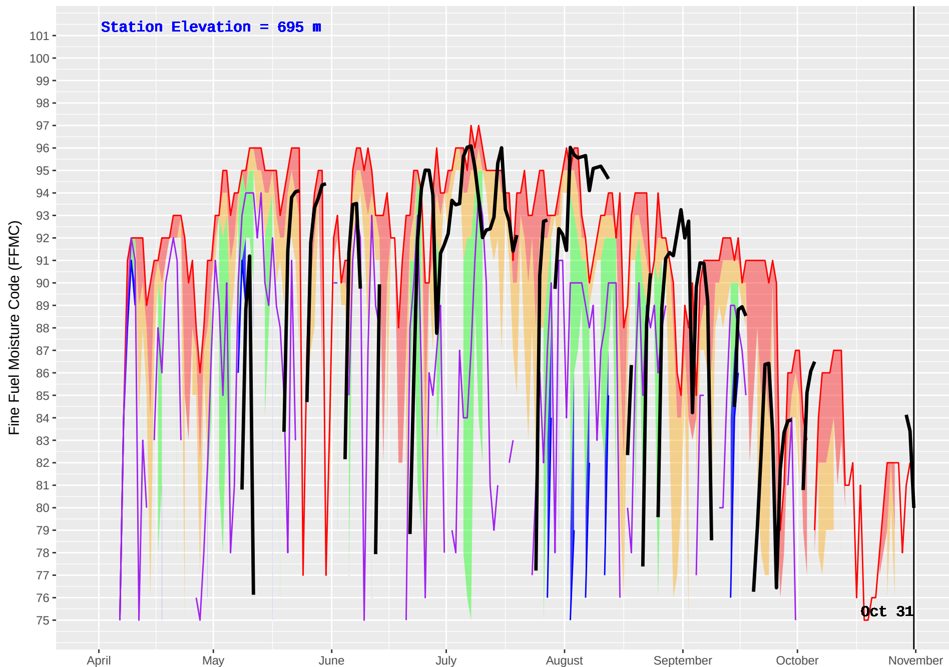
BLUE RIVER 2 (1108) : Historical (2011–2016) and Current (2017) Noon Fine Fuel Moisture Code (FFMC)
